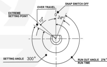
TURNING ANGLE
