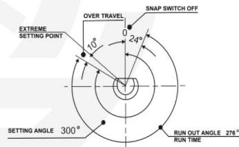
TURNING ANGLE
