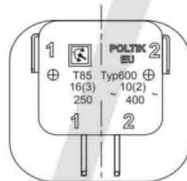
HORIZONTAL CONTACTS
